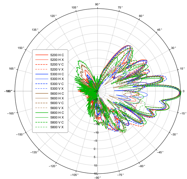
5 GHz Elevation
